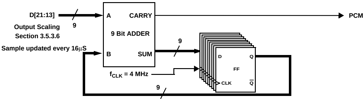
Figure 23. PCM Output Function Block Diagram
